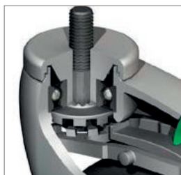
Labyrinth structure protecting the swivel bearing.
